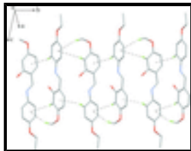
Fig. 2. Part of the crystal structure of the title compound, showing the formation of a chain along [010] generated by the C—H... \pi interactions.
